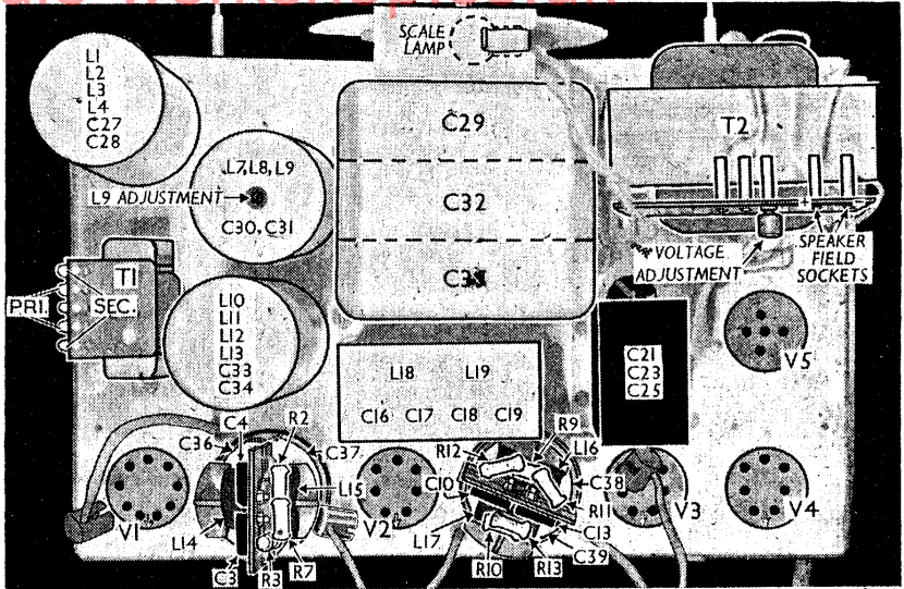
Plan view of the chassis. The adjustment screw for L9 is sunk well down below the top of the L7-L9 can. The screening cans of the IF transformers have been removed. In this illustration to permit a view of the assemblies inside them.
